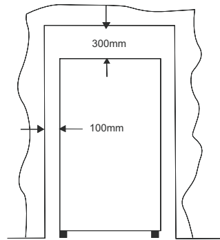
Total space required in use L5010W
